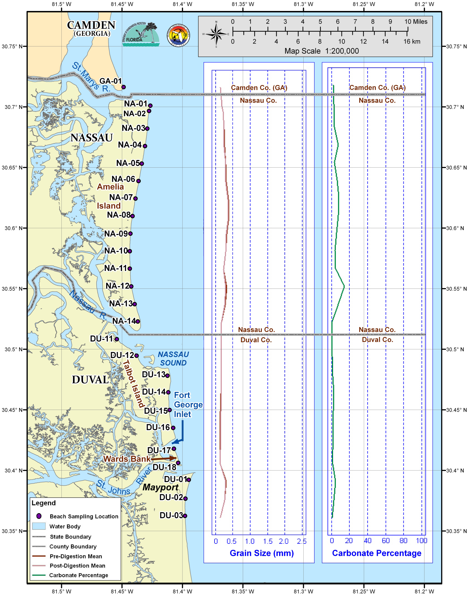
Figure 9: Grain Size and Carbonate Percentage from Amelia Island to Wards Bank
