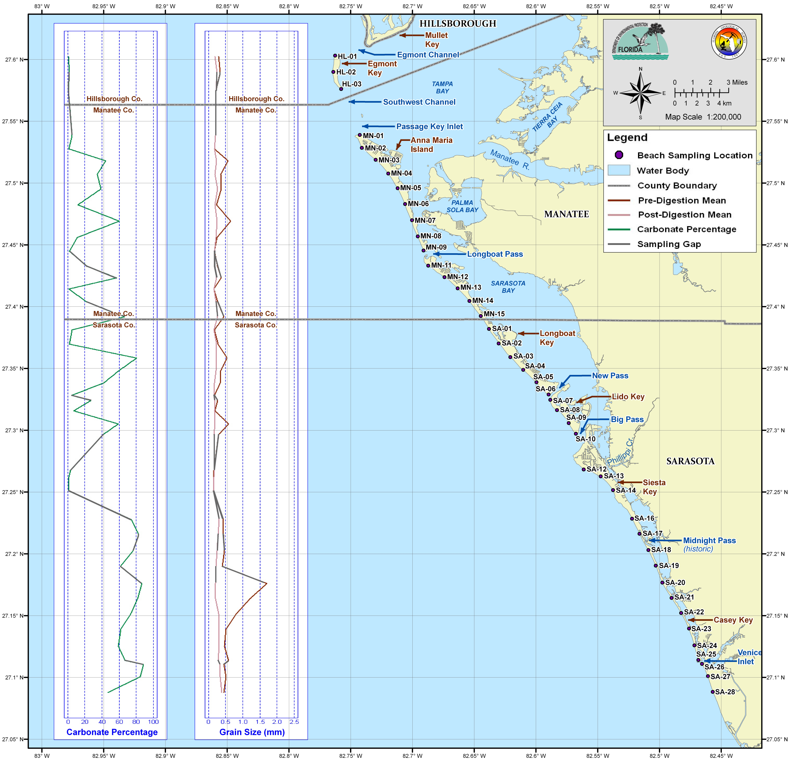
Figure 8: Grain Size and Carbonate Percentage from Egmont Key to Venice Inlet
