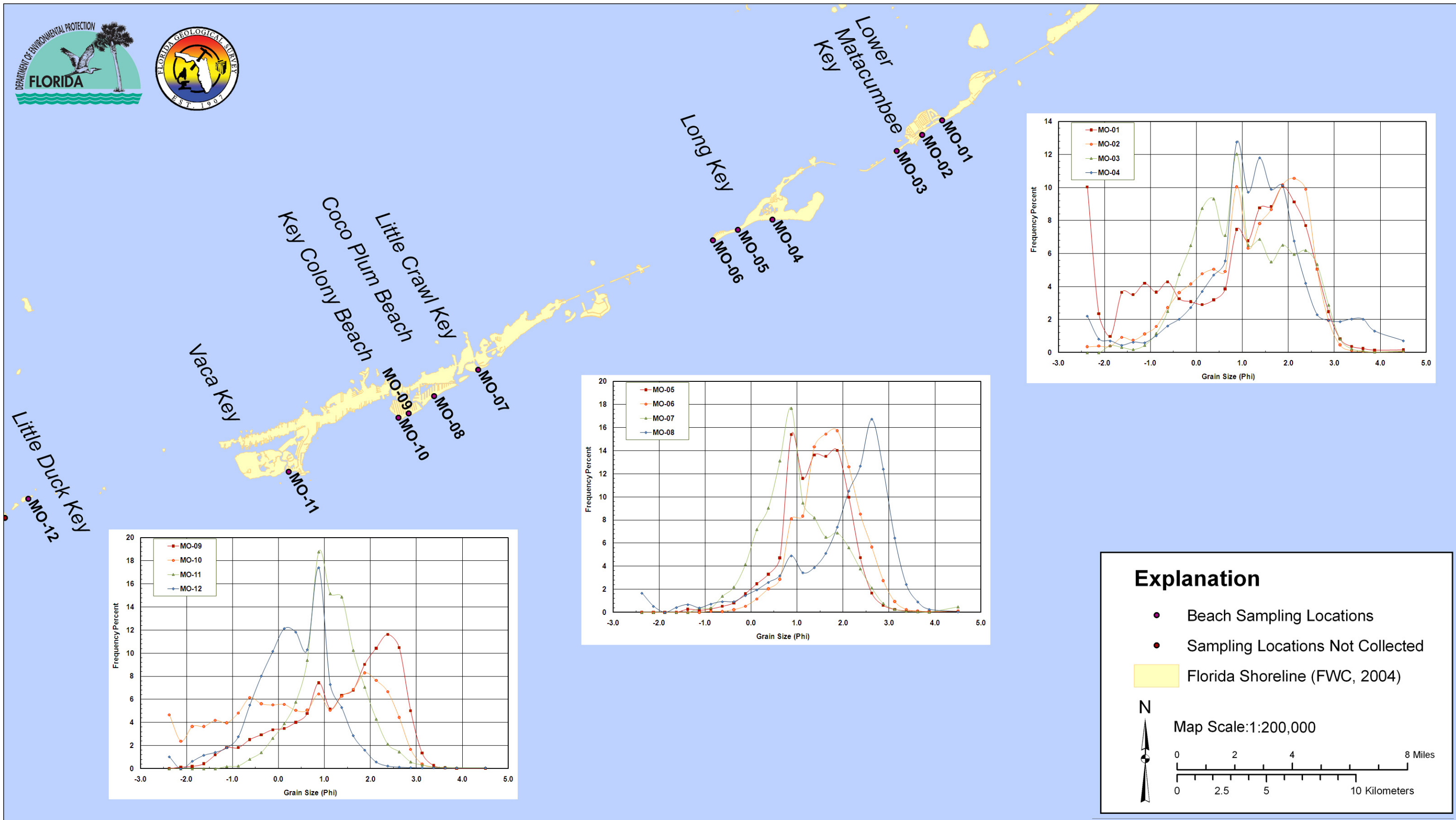
Figure 13 - Grain Size Distribution Comparisons of the Middle Keys
