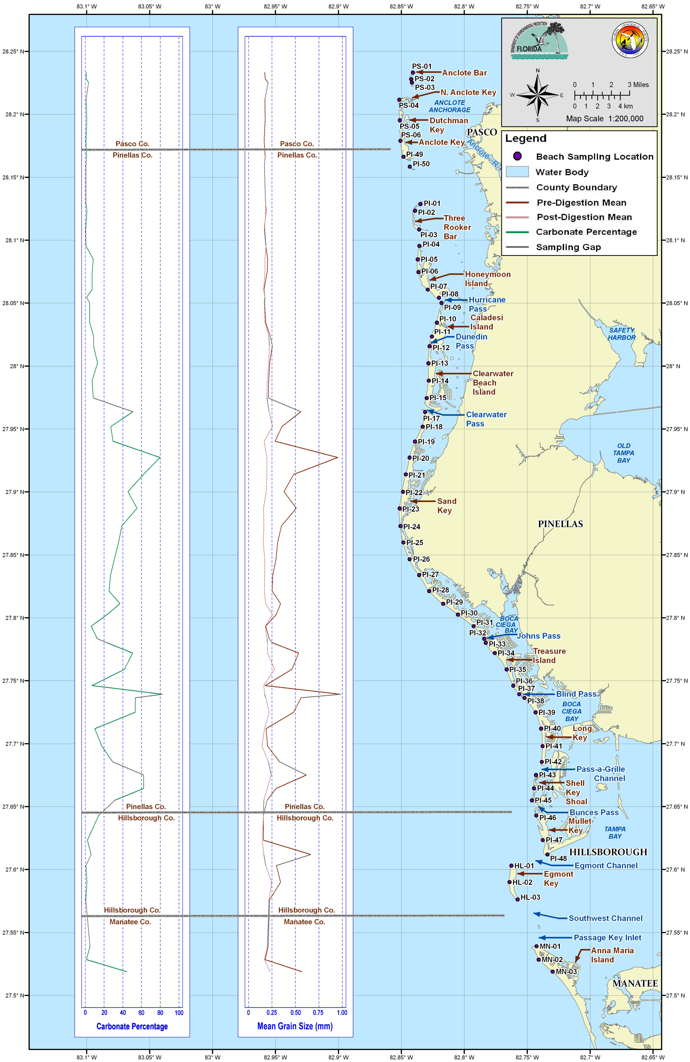
Figure 20. Mean grain size and carbonate percentage from Anclote Bar to Anna Maria Island
