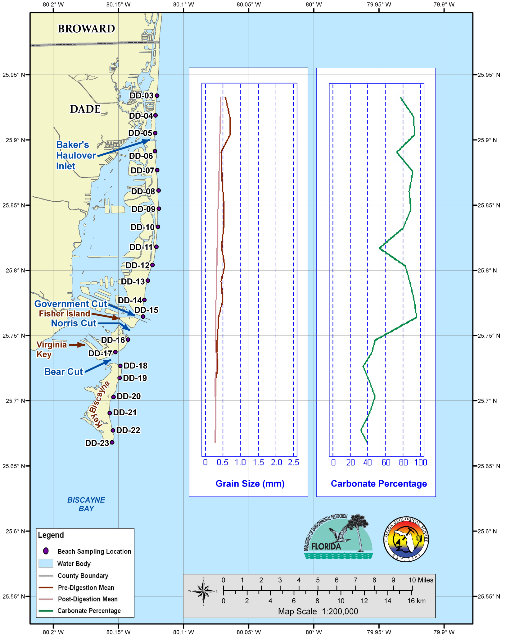
Figure 17: Grain Size and Carbonate Percentage from Baker's Haulover Inlet to Key Biscayne
