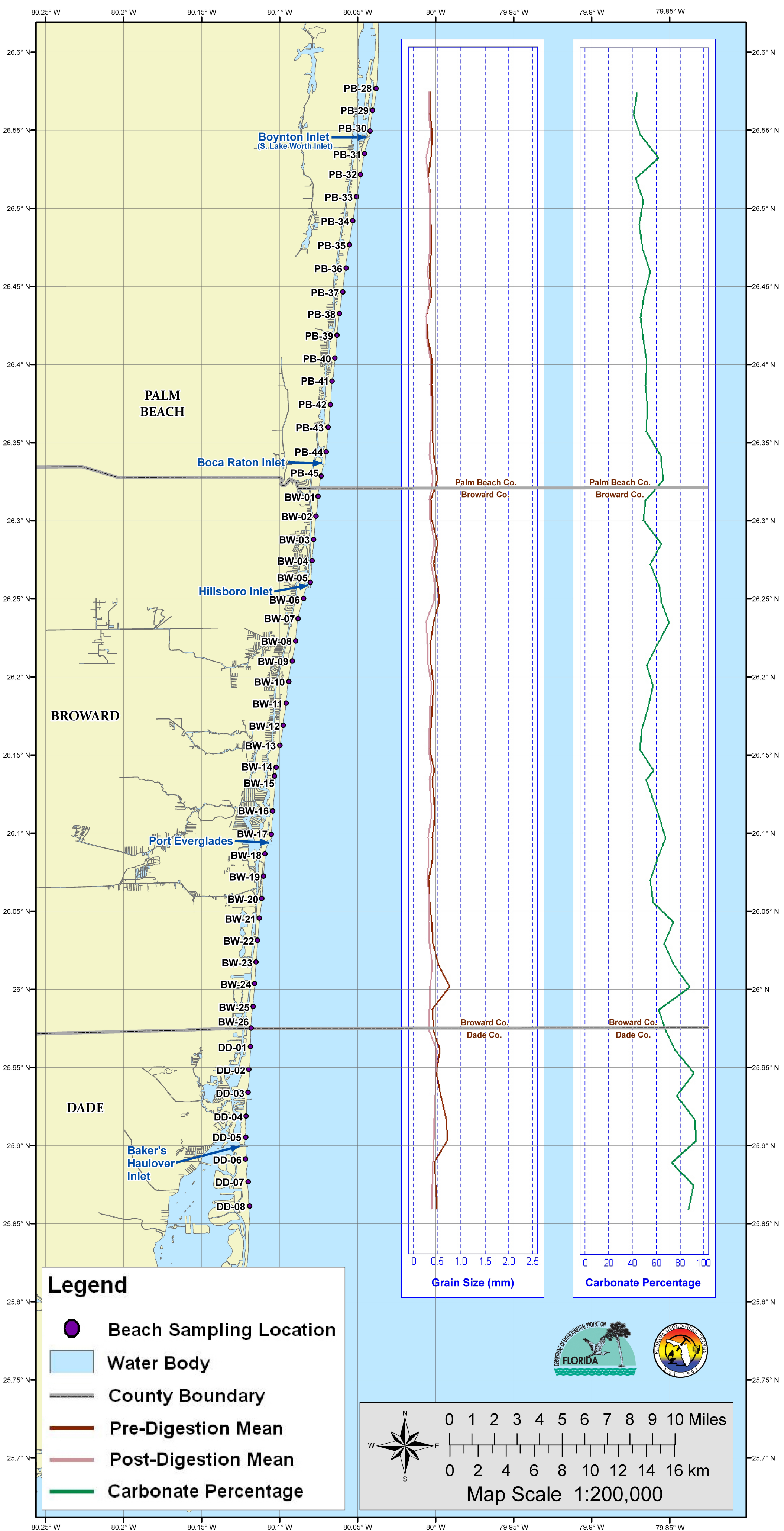
Figure 16: Grain Size and Carbonate Percentage from Boynton Inlet to Baker's Haulover Inlet
