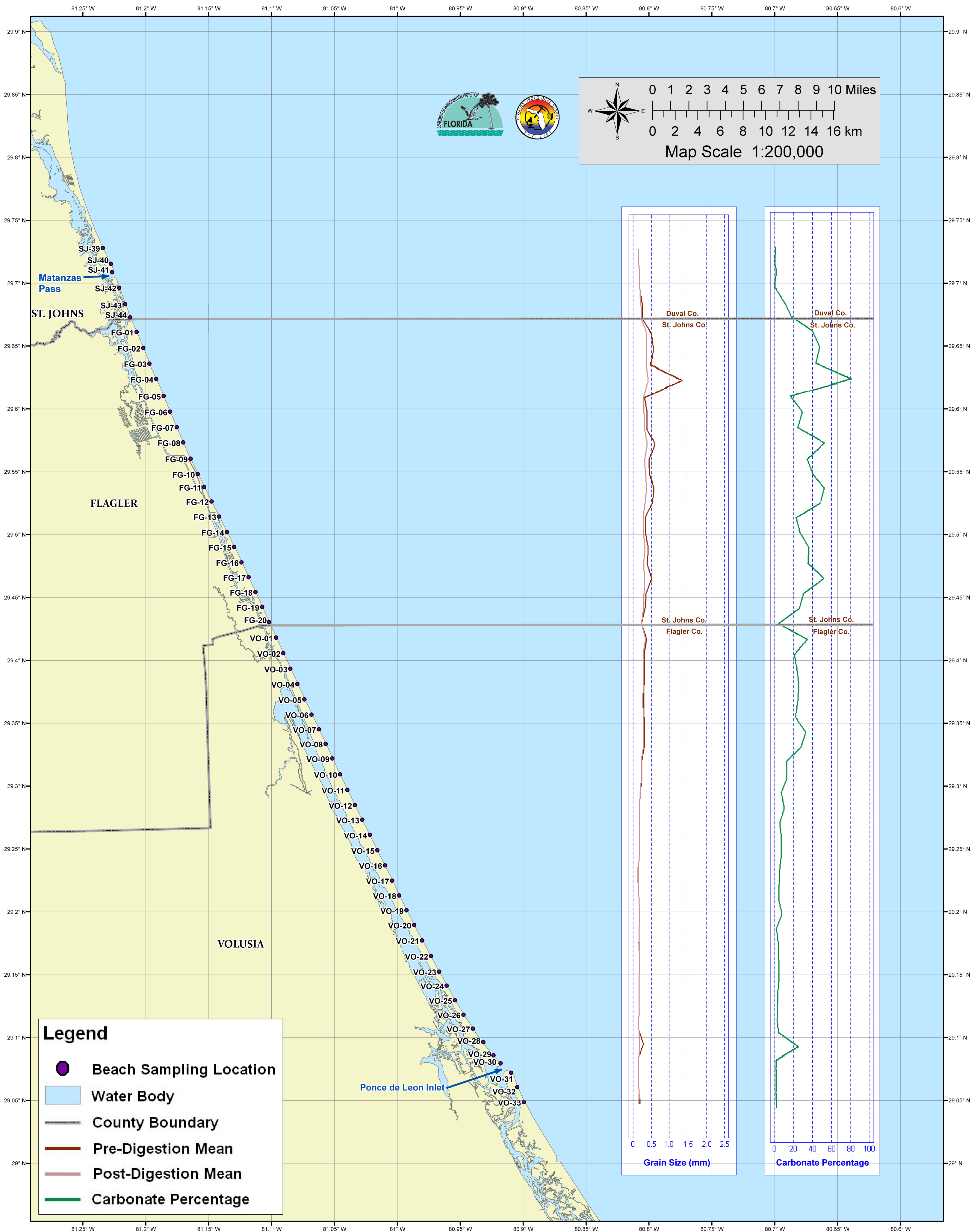
Figure 11: Grain Size and Carbonate Percentage from Matanzas Pass to Ponce de Leon Inlet
